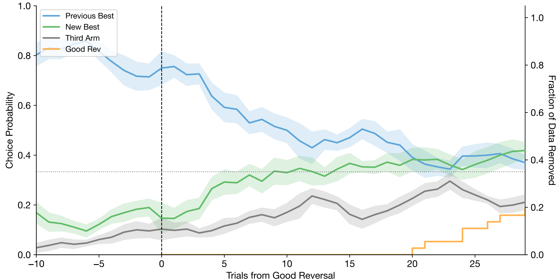
Good Reversal-Aligned Choices (mean \pm se across subjects | n=8 subjects, n=36 reversals)
